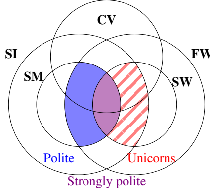
Fig. 6 A diagram of the various notions studied in this paper [1]
