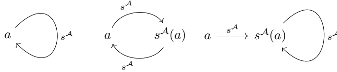
Fig. 4 Possible scenarios when \psi_{\vee} holds [1]
