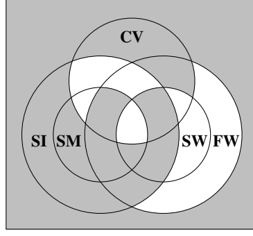
Fig. 2 A diagram of combinations over a one-sorted, empty signature: gray regions are empty [1]
