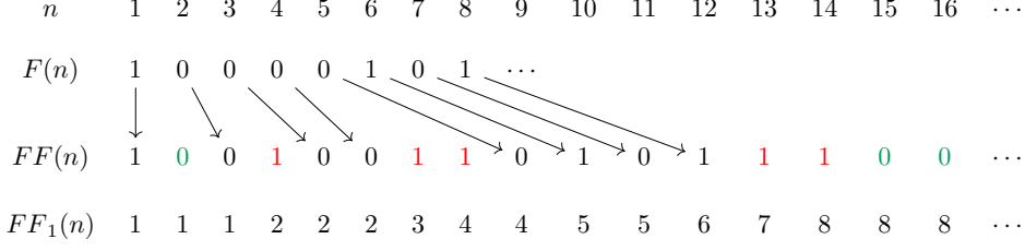
Fig. 7 A diagram for the function FF [1]
