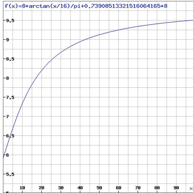
Figure 2 Graph of the luminance quantization table values.
