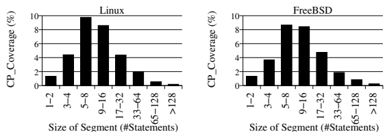
(b) The CP_Coverage with various segment sizes (# of statements)
