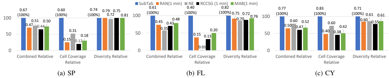
Fig. 6: Experimental results for the quality of sub-tables computed by different baselines for different datasets
