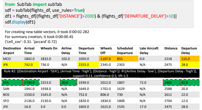
Fig. 2: Informative 10X10 sub-table for a large query result
