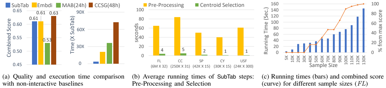
Fig. 7: Experimental results for execution times and performance
