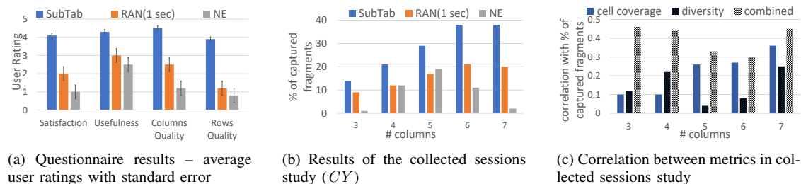
Fig. 8: Experimental results for extrinsic evaluation
