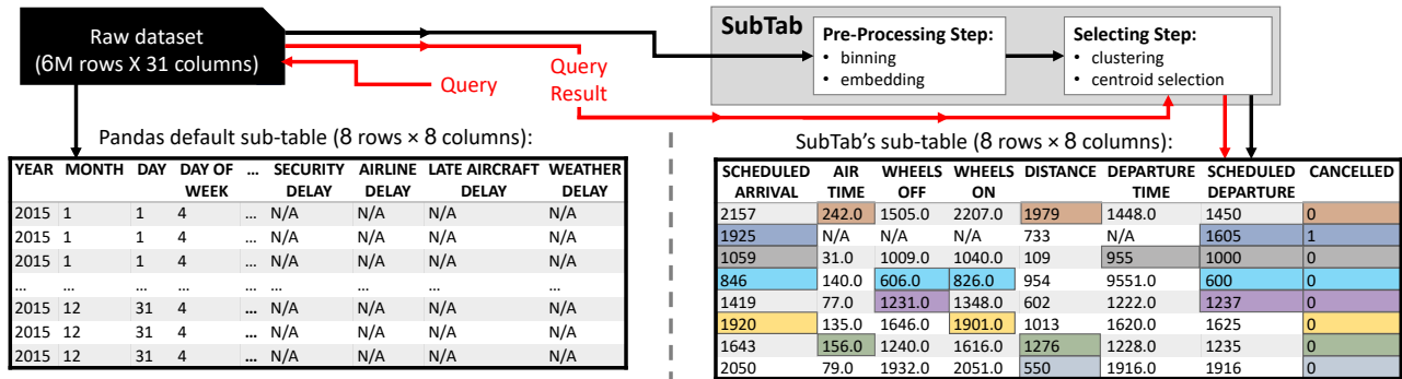
Fig. 1: System Workflow. SubTab takes as input a raw table used throughout the EDA session. The sub-table on the left is the output of the display command in Pandas, a random subset of the table’s rows and columns. The sub-table on the right is the output of SubTab, in which some of the ARs are highlighted for purposes of illustration. SubTab has two-steps: (1) Pre-Processing Step - the table is binned and embedded into vectors; (2) Selecting Step - triggered by a display of the input table or as the result of a query over the table, an informative sub-table is displayed. This is done by clustering the row and column vectors of the query result in the embedded space and selecting the centroids as representatives.
