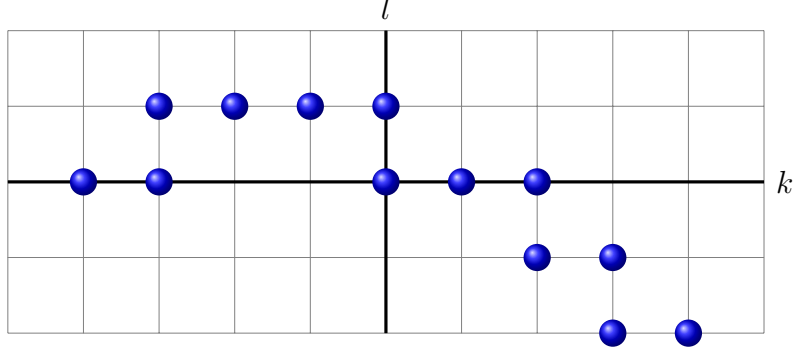
Figure 1: Possible points of G_0
