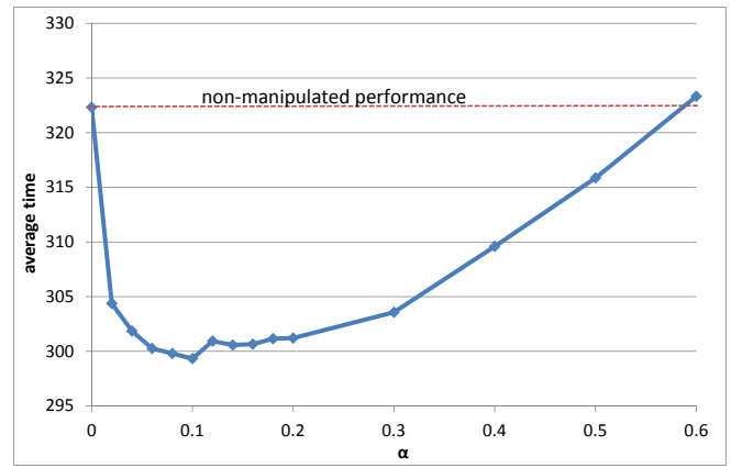
Figure 3: The effect of \alpha in “information hiding” over average performance (cross-agents)
