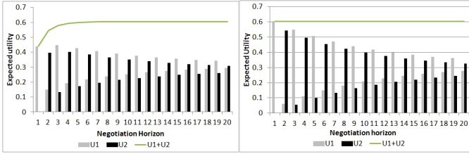
(a) Interleaved protocol (b) Non-interleaved protocol
