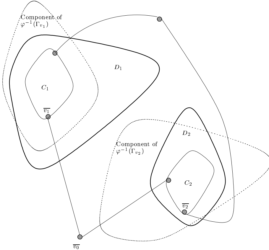
FIGURE 1. Constructing \Gamma'' .
