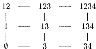
Fig. 5. Embedding in the Boolean lattice.
