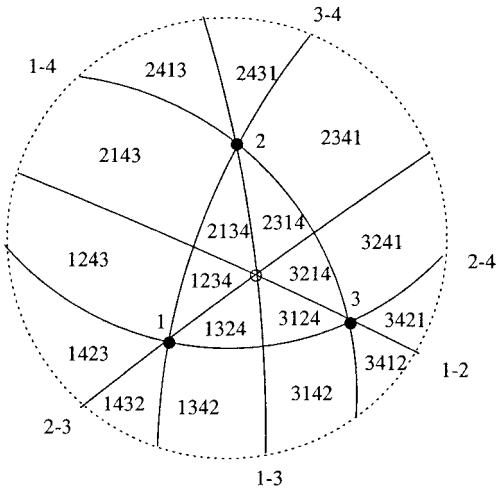
Fig. 7. The braid arrangement when n = 4 .
