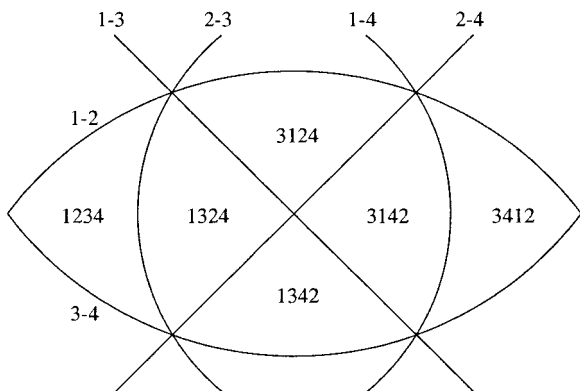
Fig. 1. A convex subset of the braid arrangement.
