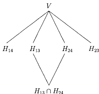
Fig. 2. The poset \mathcal{M}_0 .
