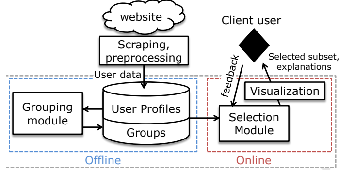
Figure 1: System Architecture
