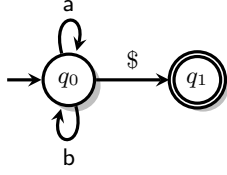
Figure 5: A_3 , a DFA with 3 choices
