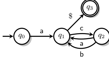
Figure 4: The A_r DFA
