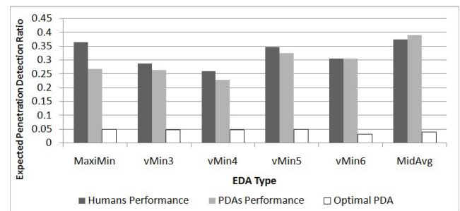
Figure 4: Results of the experiment for d = 16, t = 9 . The bars represent the expected penetration detection ratio of the robots given the actual choices of the players.
