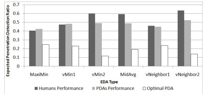
Figure 3: Results of the experiment for d = 8, t = 6 . The bars represent the expected penetration detection ratio of the robots given the actual choices of the players.
