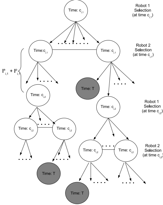
Fig. 3. An illustration of the extensive-form game tree for an LCT task. Conflict times are denoted in the nodes. Terminal nodes (total time= T ) are dark. Note that the second conflict c_{i,2} may occur at different absolute times depending on the choices of the robots at time c_{i,1} .
