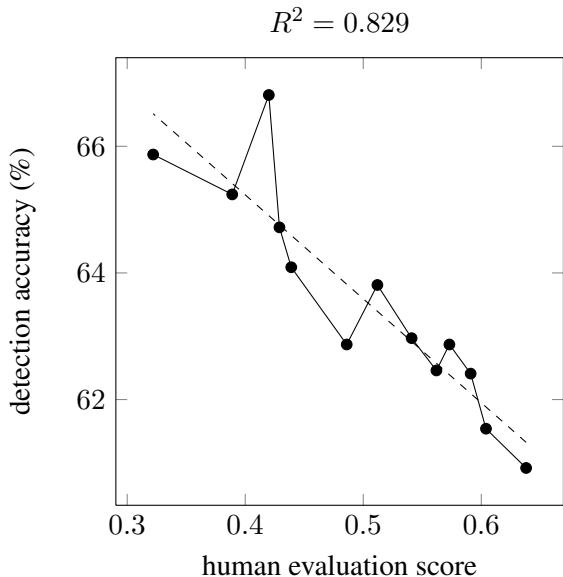
Figure 5: Correlation between detection accuracy and human evaluation scores on systems from WMT 13’ against non-reference sentences, using the syntactic CFG features described in section 4.2
