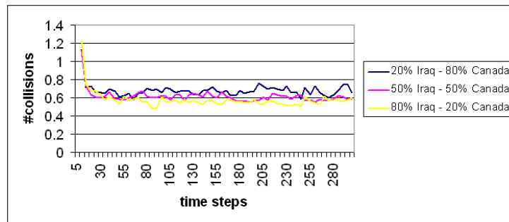
Figure 26: Impact of mix population of Iraq and Canada on #collisions
