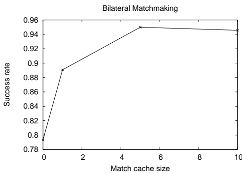
Figure 1: Success rate as a function of the matching cache size.
