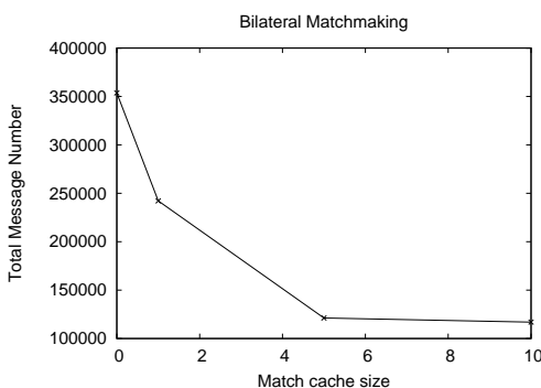
Figure 3: Number of messages as a function of the matching cache size.
