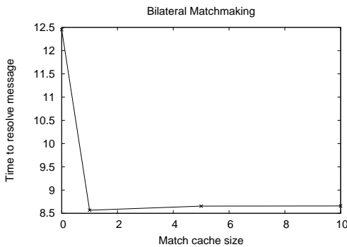
Figure 2: Time for matchmaking as a function of matching cache size.
